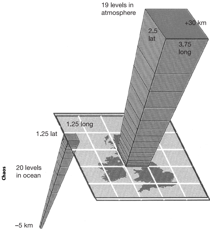
27. A schematic reflecting the way weather and climate models divide both the atmosphere and the ocean into “grid points”. Here each grid point in the atmosphere represents approximately a 250 km by 250 km square, which means that about six points account for the whole of Britain as shown above
